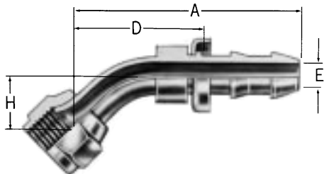
45° ELBOW FC5848S-SAE 45° swivel* FC5847S-SAE 37° (JIC) swivel FC5849S-Universal swivel†
