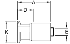
Ladish Tri-Clamp* FJ7041
