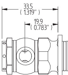
BF20-H 3/8\" Hose Banjo Fitting
