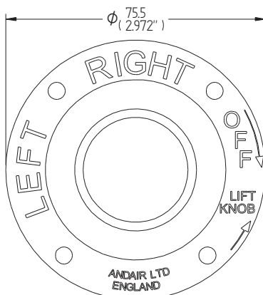
Fascia Plate
