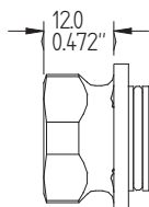
FF20 1/4\" NPT Female Fitting
