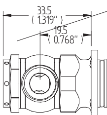
BF20 AN-6 Male Banjo Fitting
