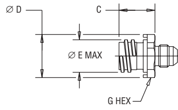
NIPPLE
