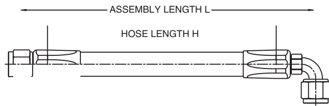
Straight-To-90° Elbow
