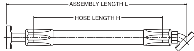
Straight-To-45° Elbow
