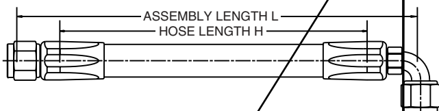
Straight-To-90° Elbow
