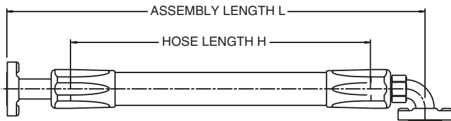
Straight-To-90° Elbow
