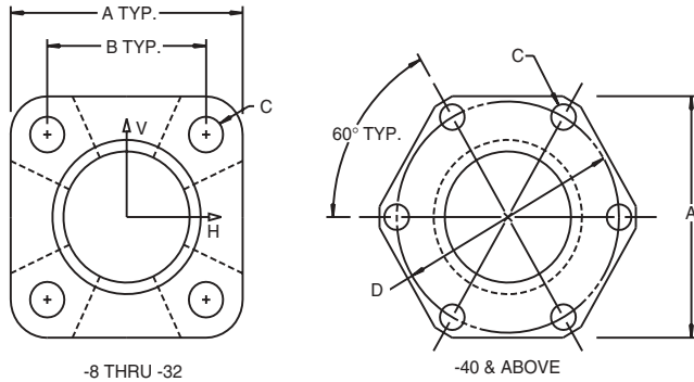
MS20756 Flange
