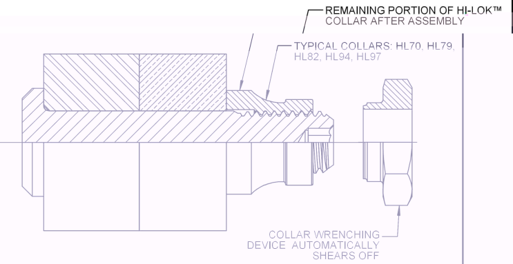
HI-LOK™ PIN AND COLLAR AFTER ASSEMBLY
