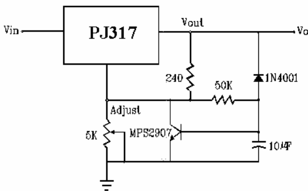
FIGURE 22-SLOW TURN-ON REGULATOR
