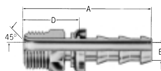
SAE 45° inverted male flare 4740-
