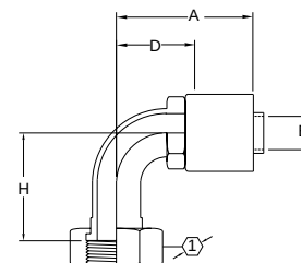
ORS® Swivel 90° elbow (long) FJ9715/FJ9899
