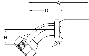
45° elbow universal swivel FC5936 SAE 37° (JIC) swivel FC5813
