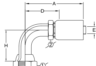
90° elbow universal swivel FC5937 SAE 37° (JIC) swivel FC5814
