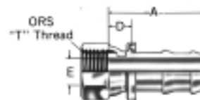
ORS Swivel Straight FJ7044-
