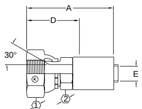
30° swivel — Metric threads Special Komatsu FJ7188
