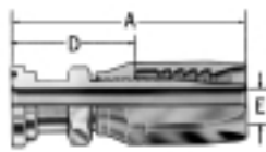
Code 61 SAE J518 Straight split flange FC5135-
