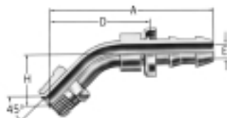
SAE male inverted flare 45° elbow 190944-
