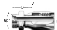
BSP male 07.340-
