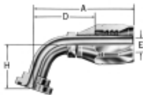
60° split flange
