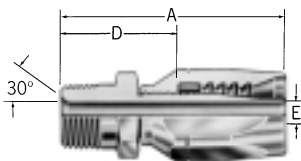
Male pipe 4722-
