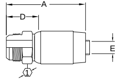
SAE 37° (JIC) male flare FJ9917
