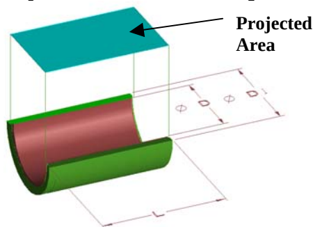
Figure 3, (Non-flanged Journal)
