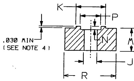
ROLLER BASE
